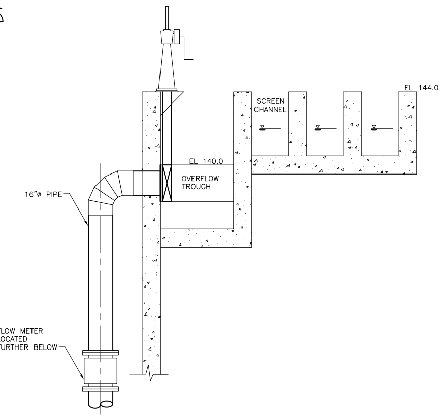
SECTION A 3/8" = 1'-0" H-2
