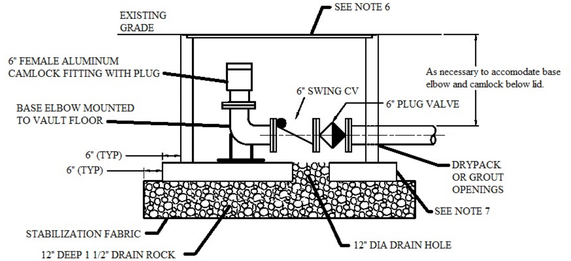
D SECTION
