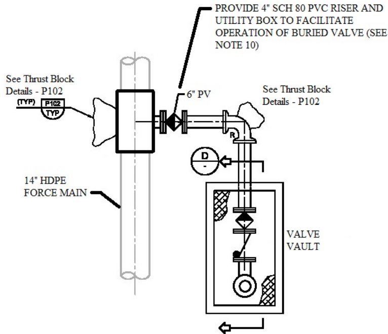
A PLAN
